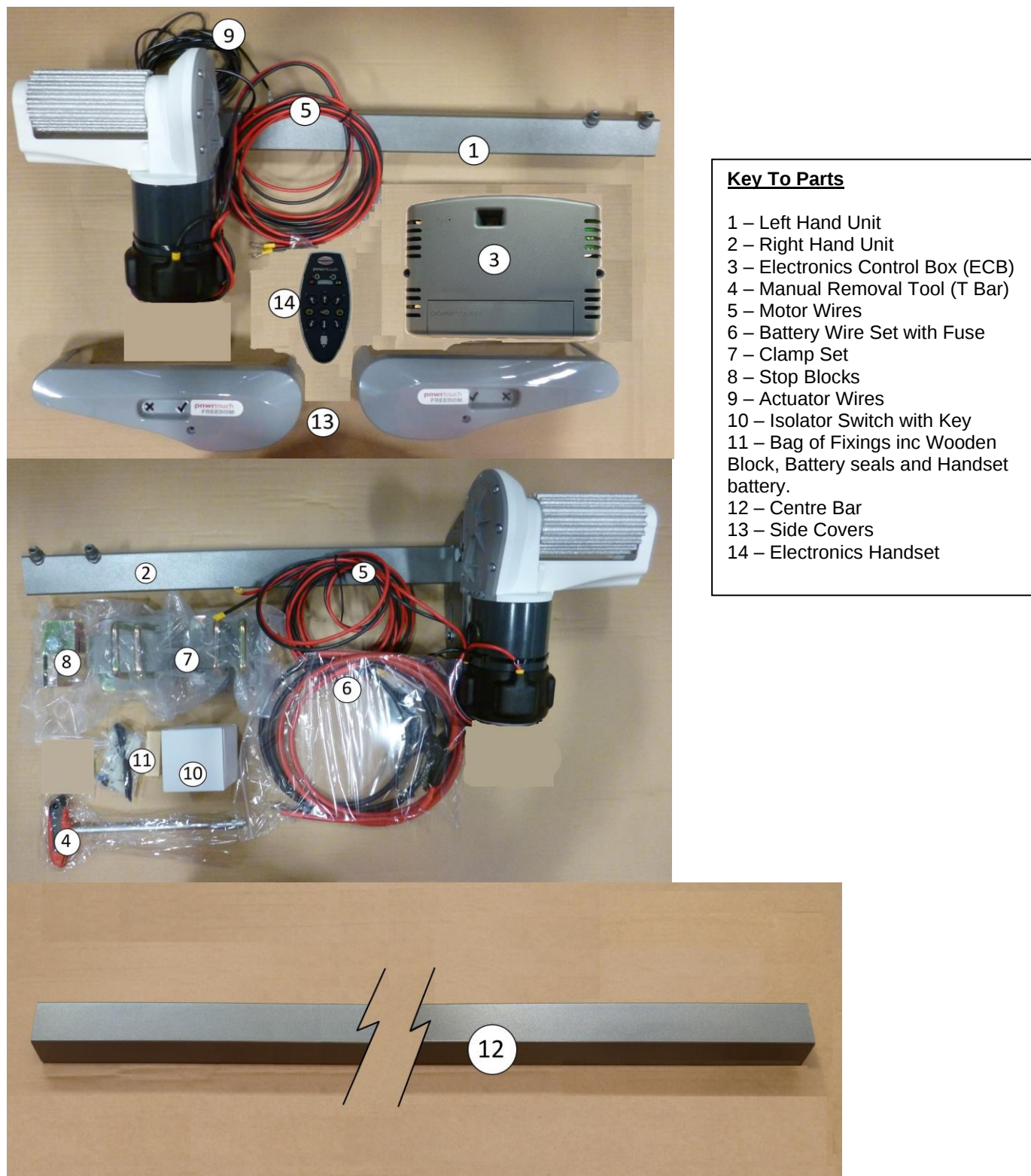
Fig 1. Pictures Showing Component Parts
